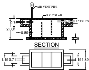
SEPTIC TANK PLAN
