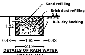
DETAILS OF RAIN WATER HARVESTING Dwg:1A
