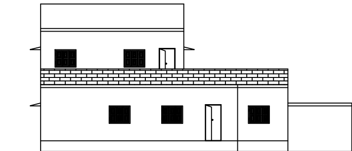
FRONT ELEVATION
