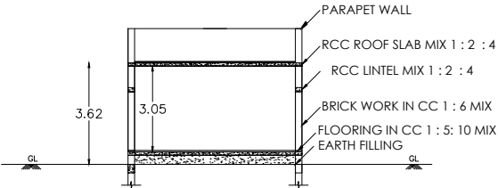
SECTION ON AB & ( HALF ELEVATION)
