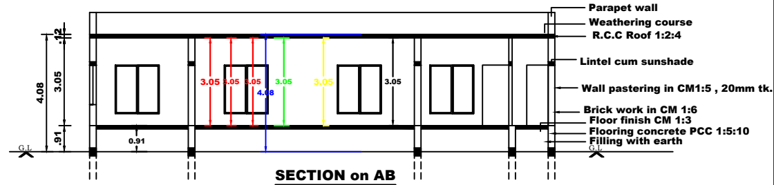
SECTION on AB
