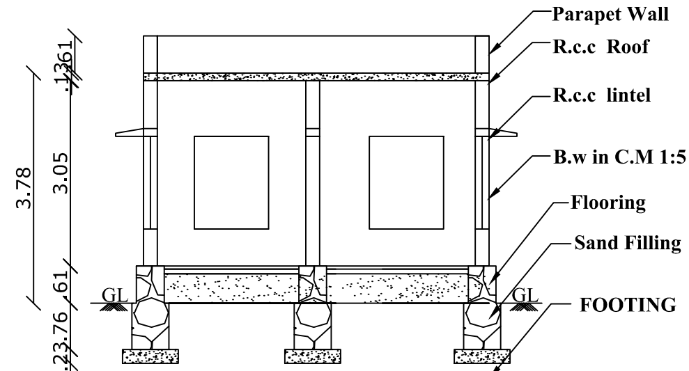
SECTION-AB
