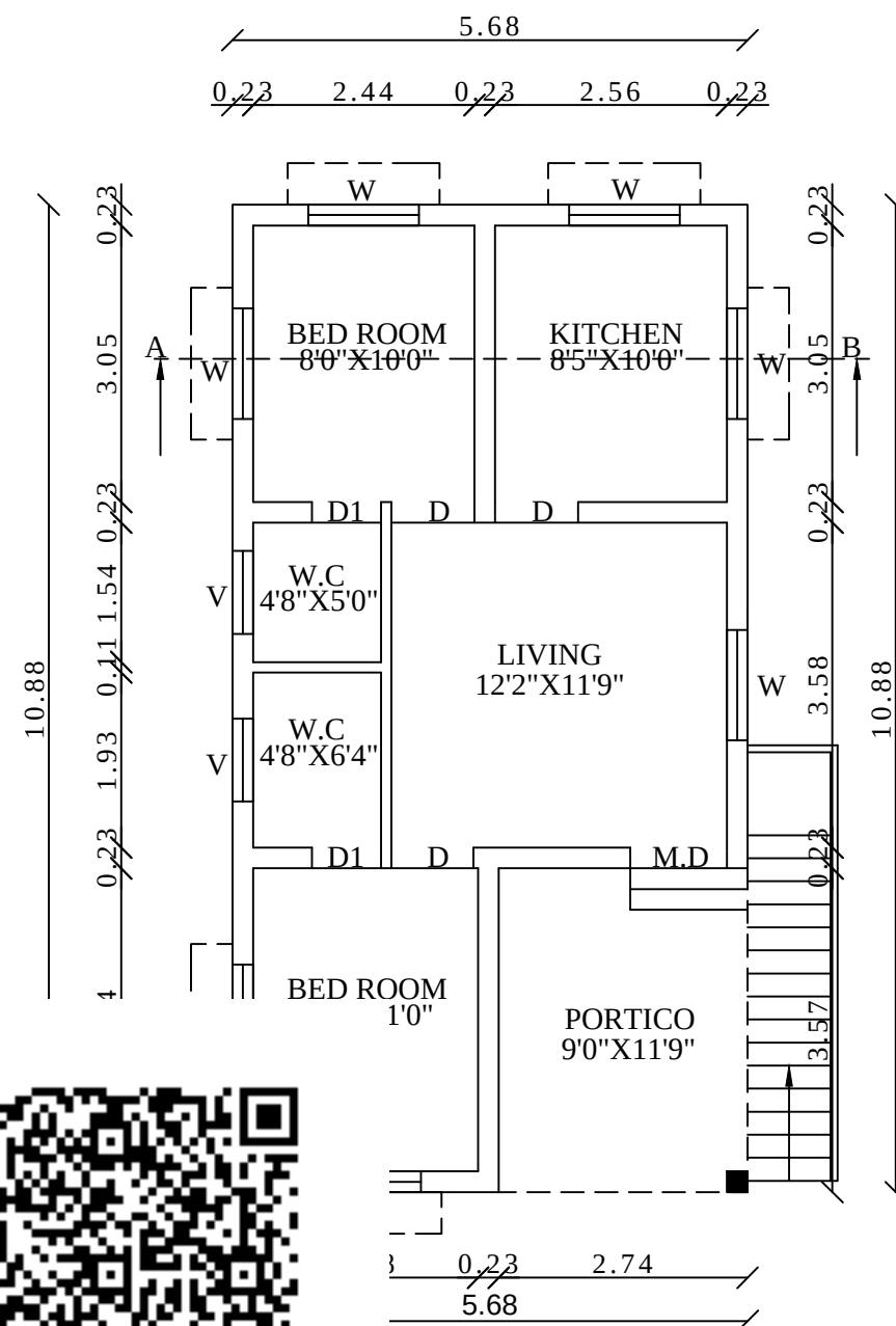
PLAN
