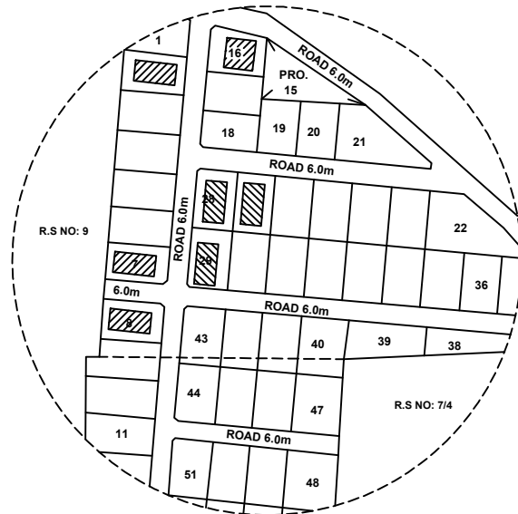
TOPO PLAN
