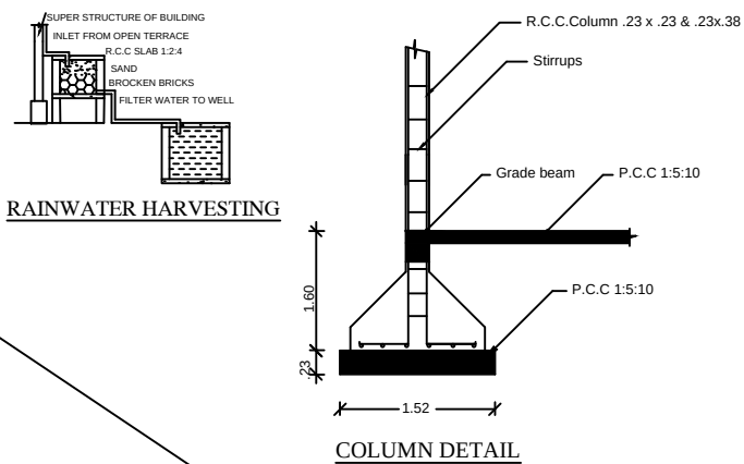
COLUMN DETAIL
