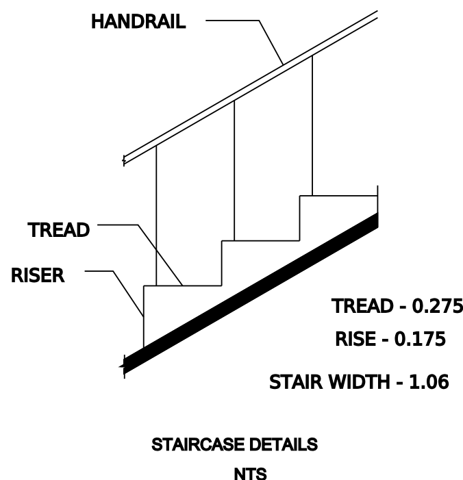
STAIRCASE DETAILS NTS
