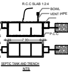
SEPTIC TANK AND TRENCH
