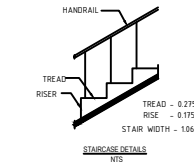
STAIRCASE DETAILS
