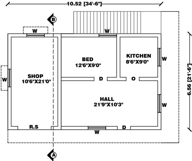
FIRST FLOOR PLAN (SHOP & HOUSE BUILDING)
