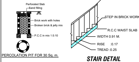
STAIR DETAIL
