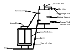
Details Of Solar Water Heater (NTS)
