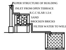
Rainwater harvesting
