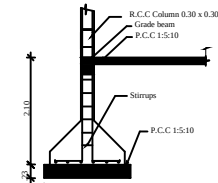
Column Detail
