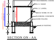
SECTION ON - AA
