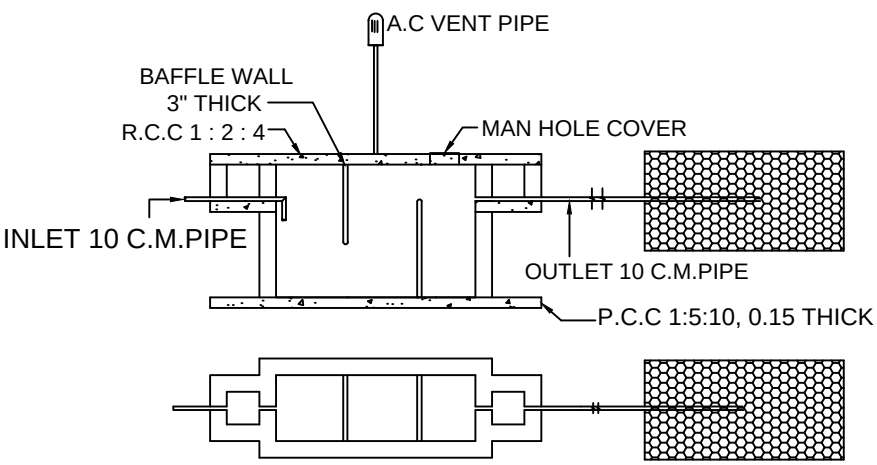
SEPTIC TANK & TRENCH
