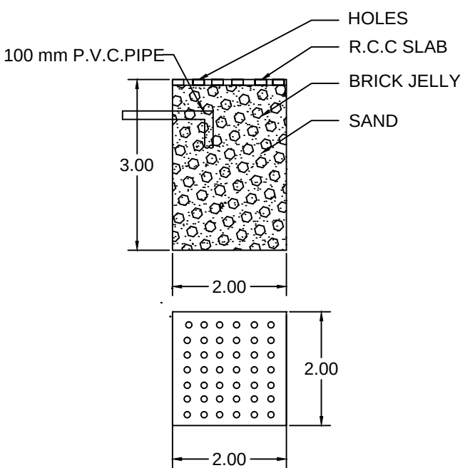
RAIN WATER COLLECTING TANK
