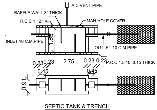
SEPTIC TANK & TRENCH
