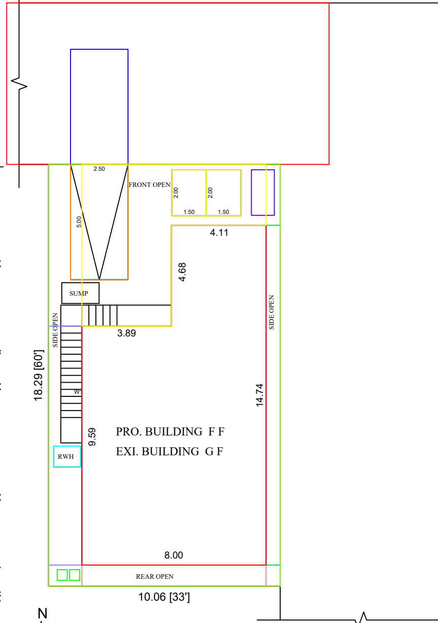
SITE PLAN
