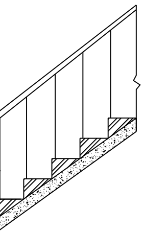
STAIR DETAIL
