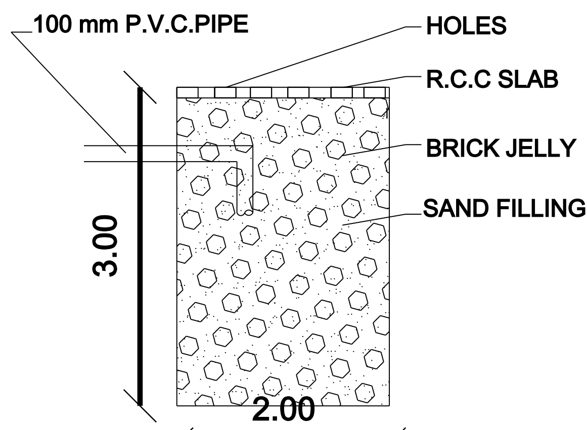
SECTION OF RAIN WATER COLLECTING TANK
