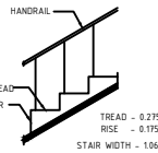
STAIRCASE DETAILS
