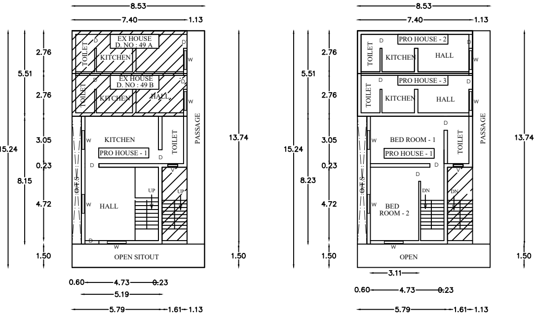
EXISTING & PROPOSED GROUND FLOOR PLAN
