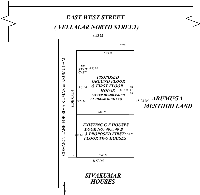
SITE PLAN
