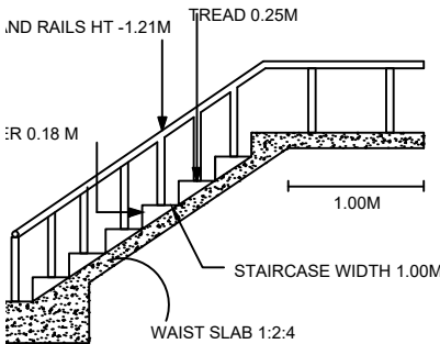
STAIRCASE DETAILS
