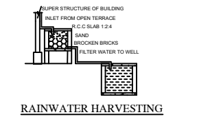
RAINWATER HARVESTING
