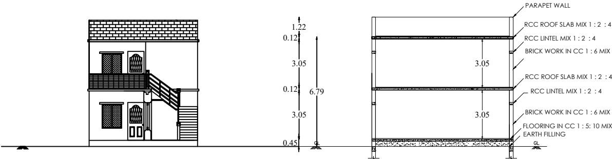
SECTION ON AB & ( HALF ELEVATION)
