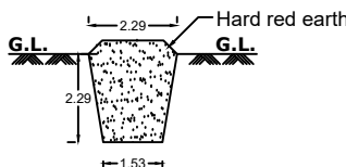
TRIAL PIT (Scale 1:100)
