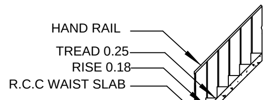
STAIRCASE DETAILS
