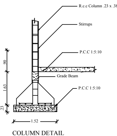
COLUMN DETAIL
