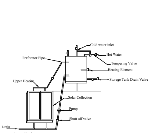
Details Of Solar Water Heater (NTS)
