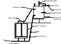
Details Of Solar Water Heater (NTS)
