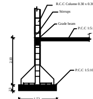
Column Detail
