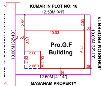
SITE PLAN (SCALE:1:200)
