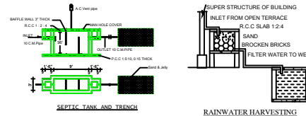
SEPTIC TANK AND TRENCH
