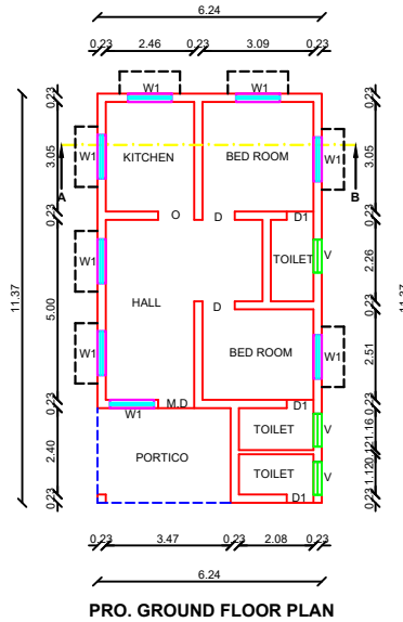
PRO. GROUND FLOOR PLAN
