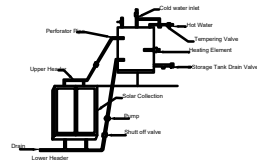
Details of Solar water Heater (NTS)
