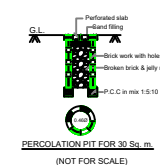
RAINWATER HARVESTING
