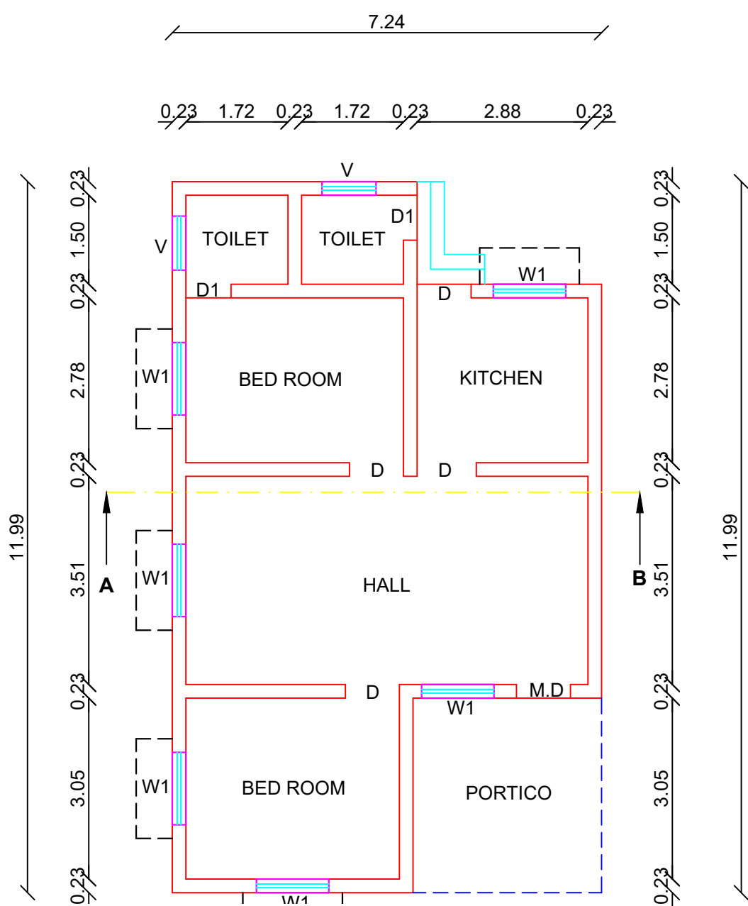
3.18 FLOOR PLAN
