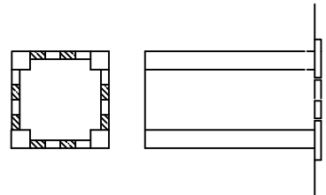
PLAN & SECTION OF RAIN WATER COLLECTION WELL
