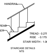
STAIRCASE DETAILS NTS
