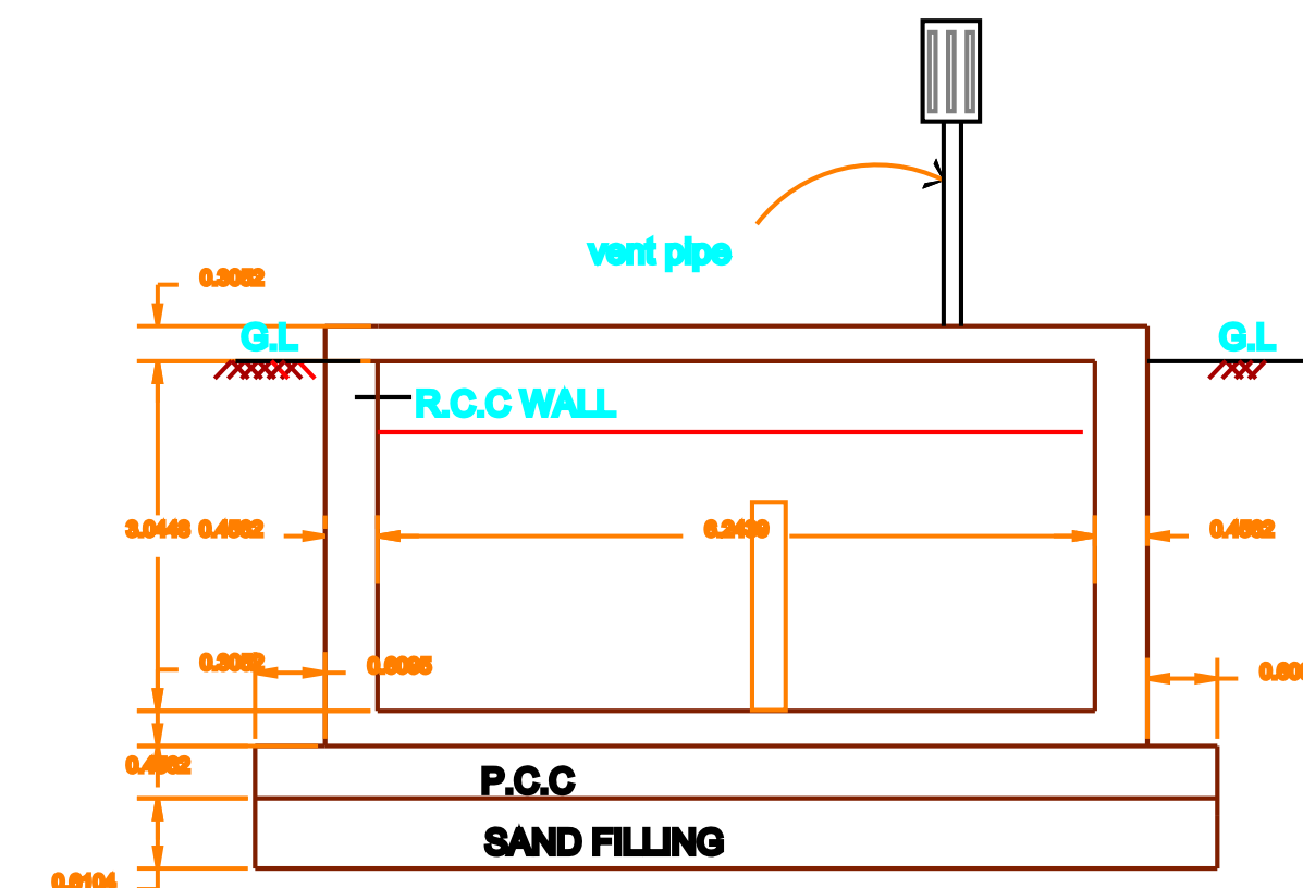
SECTION ON D-D
