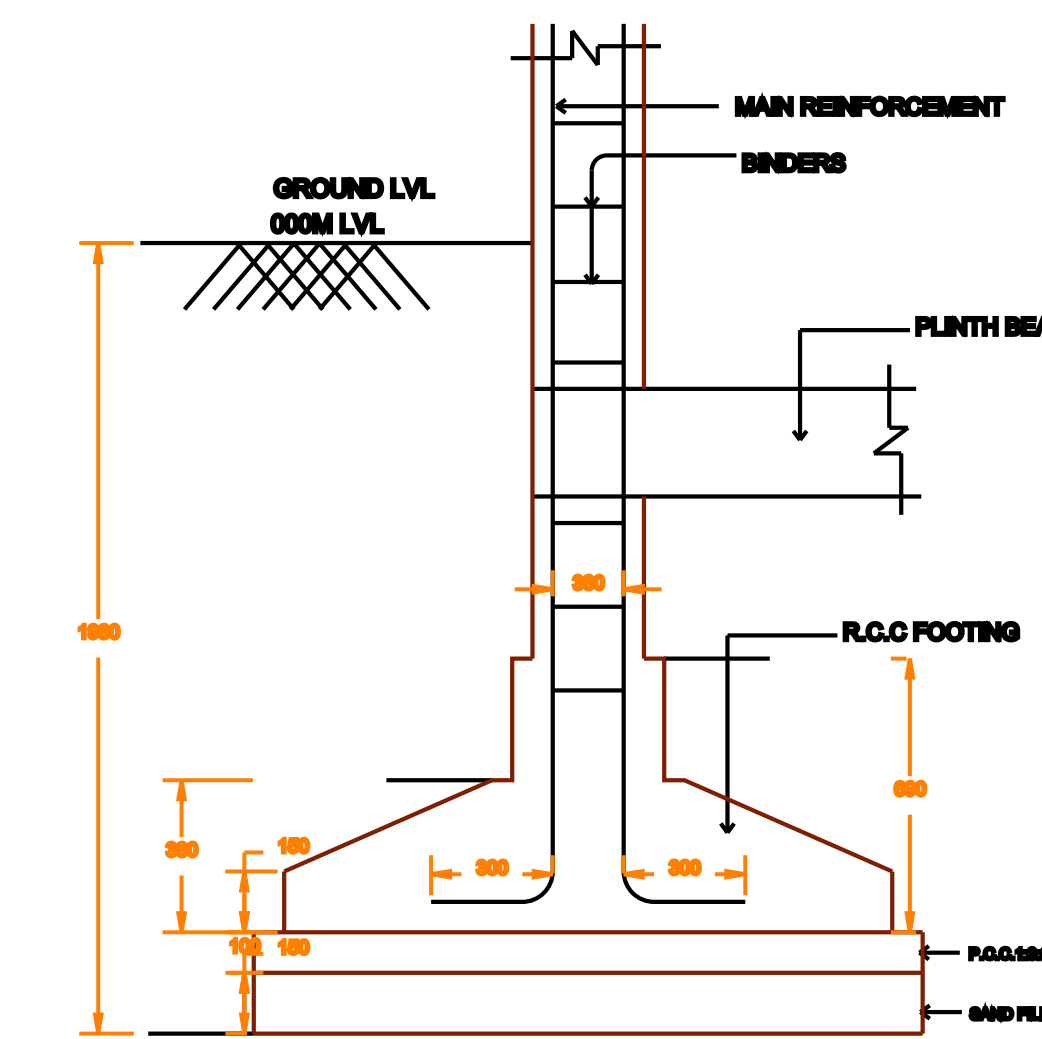
TYPICAL SECTION OF R.C.C COLUMN FOUNDATION
