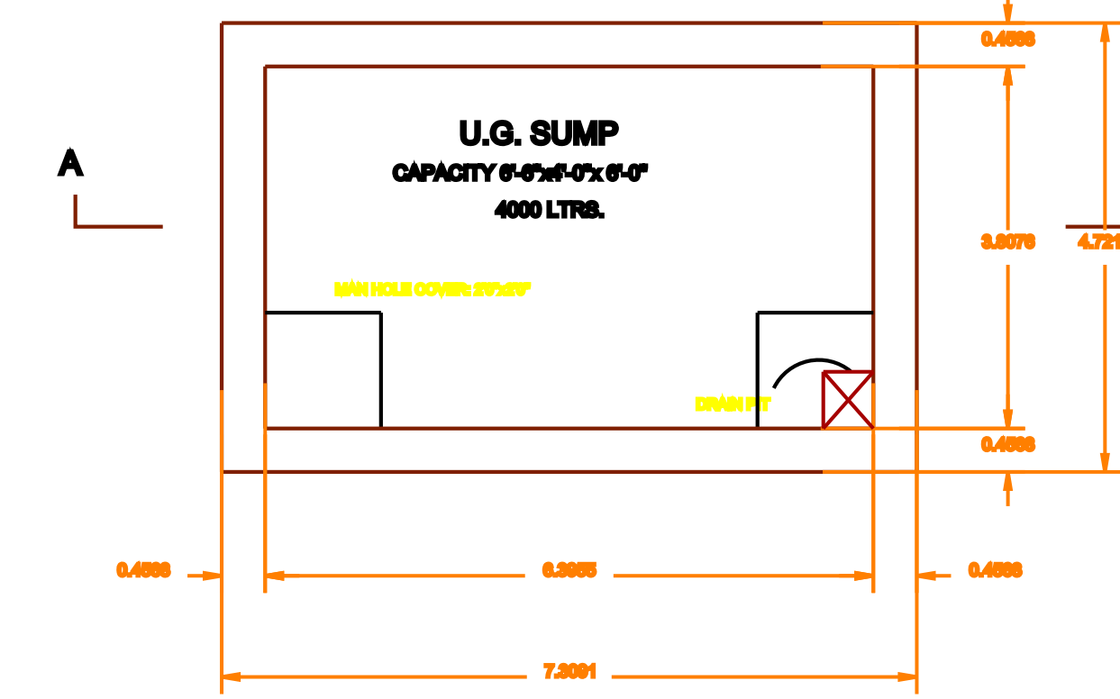
SUMP DETAIL
