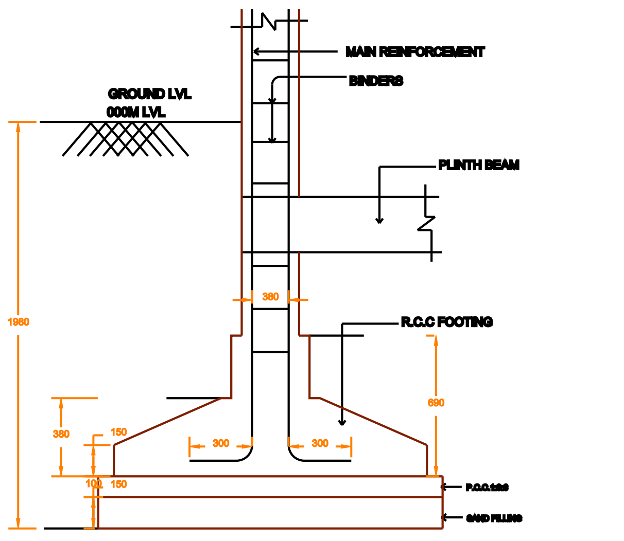
TYPICAL SECTION OF R.C.C COLUMN FOUNDATION SCALE: 1"=2'0"
