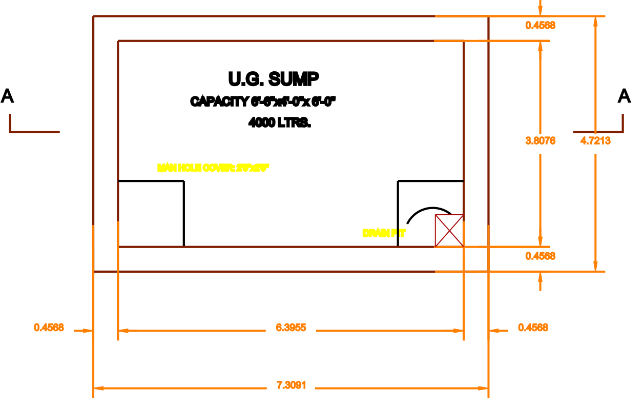
SUMP DETAIL
