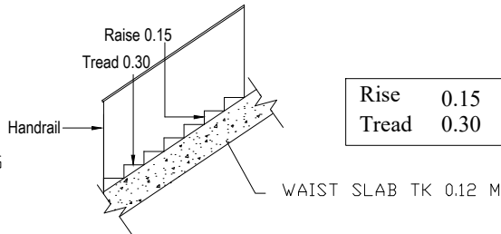
STAIRCASE DETAIL
