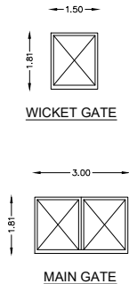
MAIN GATE
