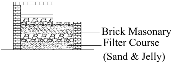
SECTION OF RECHARGE TRENCH METHOD
