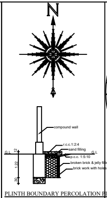
PLINTH BOUNDARY PERCOLATION PIT
