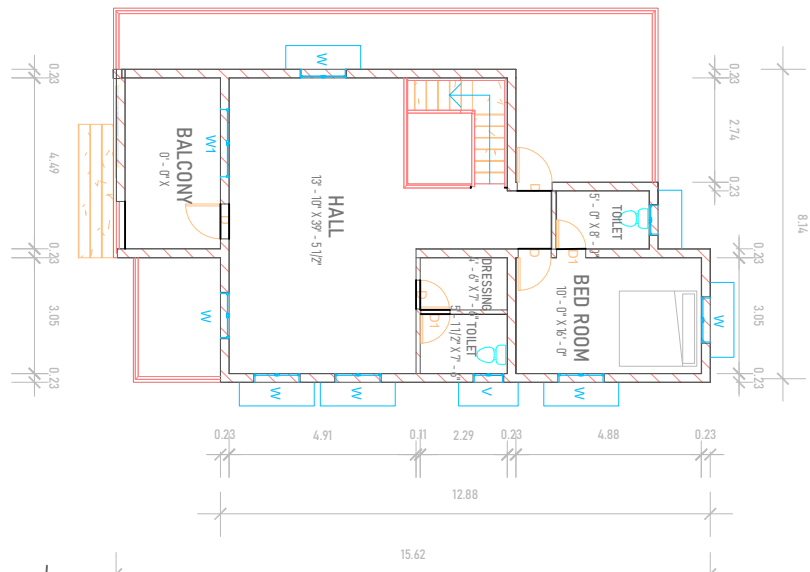
PRO FIRST FLOOR
