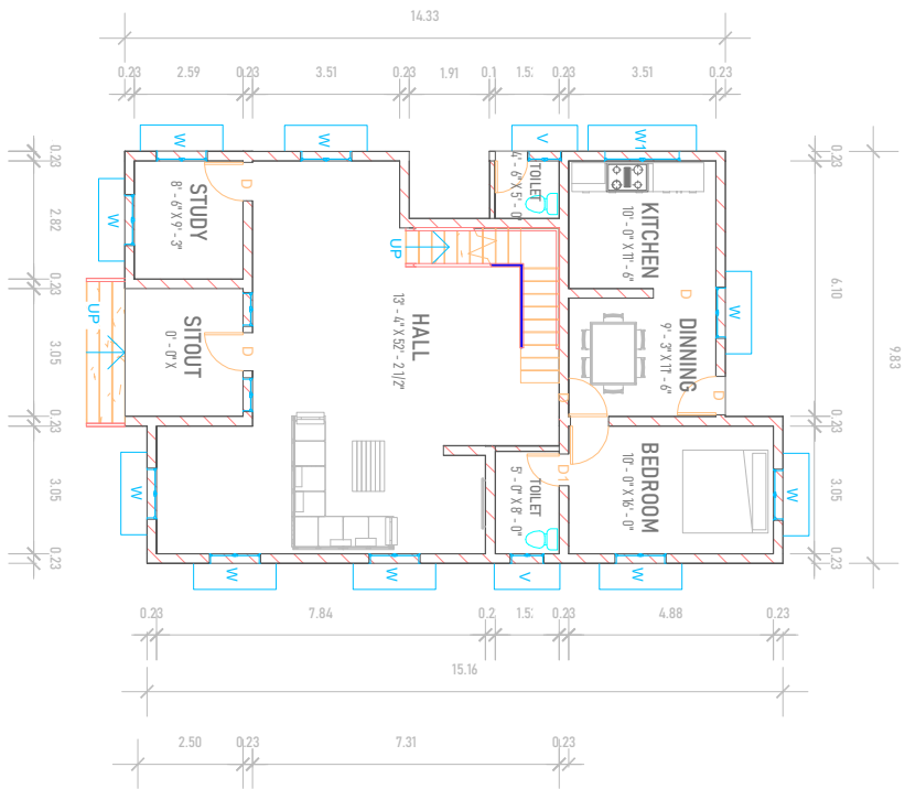
PRO GROUND FLOOR
