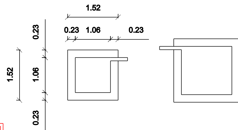
DETAILS OF FILTER BED & WELL
