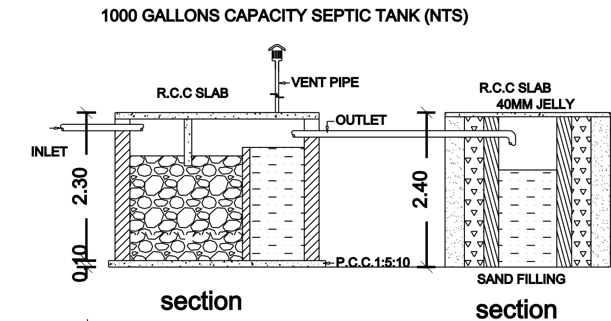
1000 GALLONS CAPACITY SEPTIC TANK (NTS)
