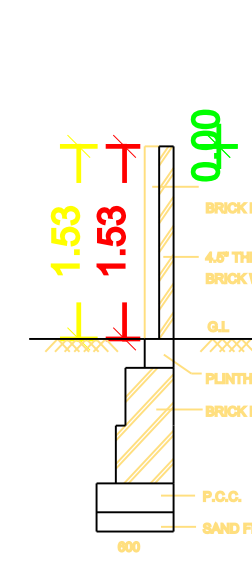
COMPOUND WALL DETAIL
