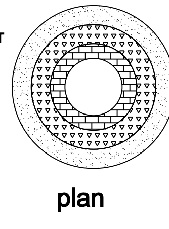
LEACH WELL DETAIL
