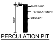
PERCOLATION PIT
