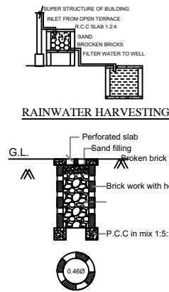
RAINWATER HARVESTING PERCOLATION PIT FOR 30 Sq. m. (NOT FOR SCALE)
