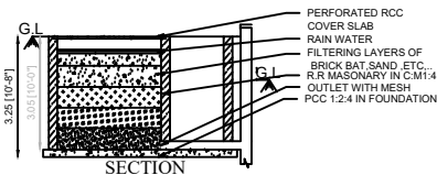
RAIN WATER HARVESTING OF RECHARGE TRENCH METHOD
