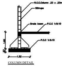
COLUMN DETAIL
