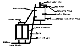
Details Of Solar Water Heater (NTS)
