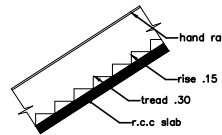
STAIR
