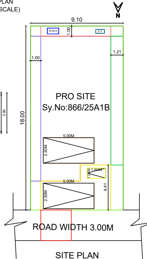
SITE PLAN
