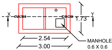
SEPTIC TANK
