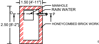
PLAN RAIN WATER HARVESTING
