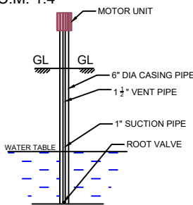
SEC.OF BOREWELL
