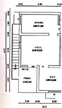
PRO. GROUND FLOOR F
