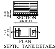
SEPTIC TANK DETAILS
