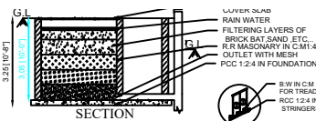
RAIN WATER HARVESTING OF RECHARGE TRENCH METHOD
