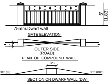
SECTION ON DWARF WALL (DW)
