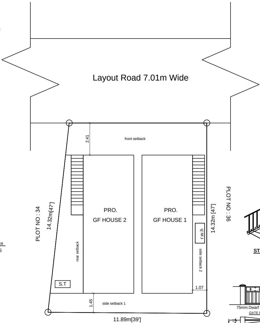
SITE PLAN
