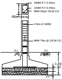
RCC COLUMN DETAILS
