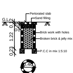
PERCOLATION PIT FOR 30 Sq. m. (Scale:- 1:50)
