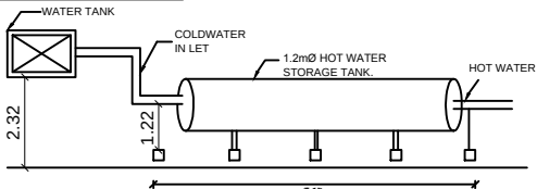
SOLAR WATER HEATING SWHS DETAIL
