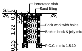
PERCOLATION PIT FOR 30 Sq. m. (Scale:- 1:50)
