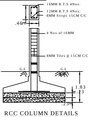
RCC COLUMN DETAILS
