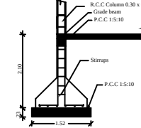
Column Detail
