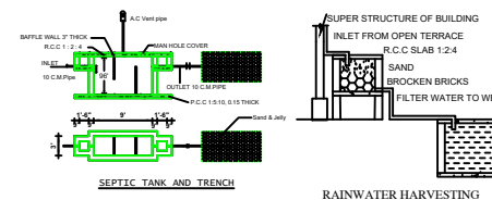
RAINWATER HARVESTING
