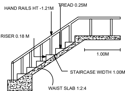
STAIRCASE DETAILS
