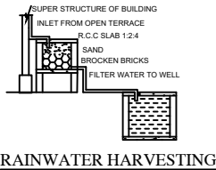
RAINWATER HARVESTING
