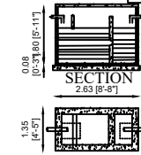
SEPTIC TANK DETAILS
