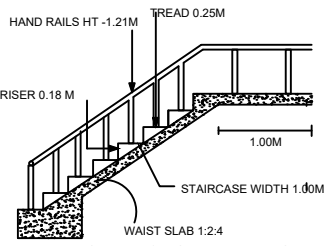
STAIRCASE DETAILS
