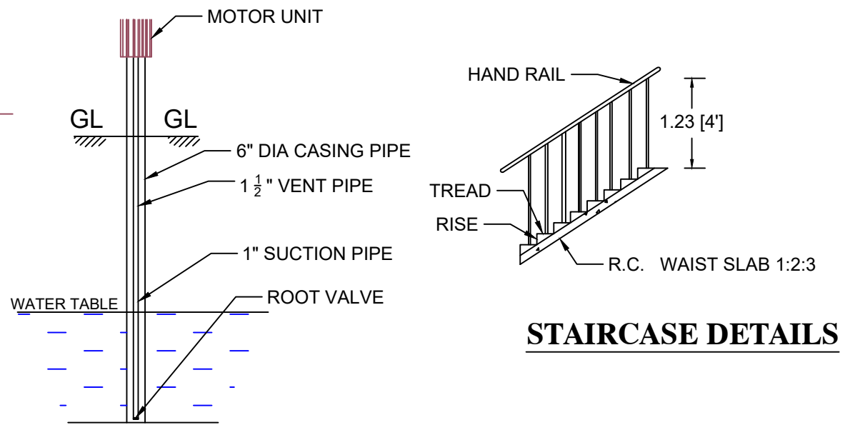
SEC.OF BOREWELL
